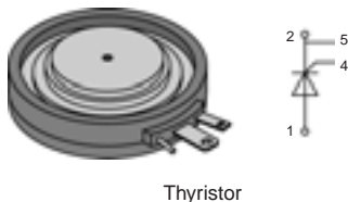
Thyristor
