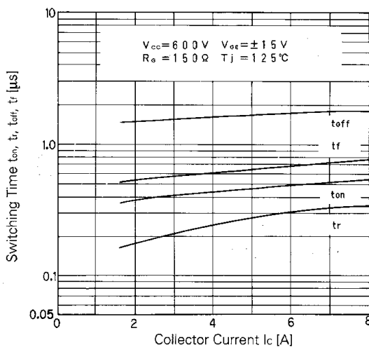
Switching Time
