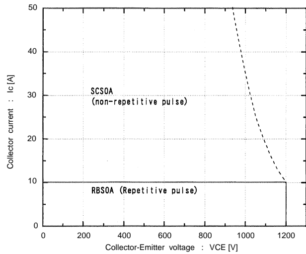
Reversed biased safe operating area +V_{GE}=15V, -V_{GE} \leq 15V, T_j \leq 125^\circ C, R_G \geq 120 \text{ ohm}
